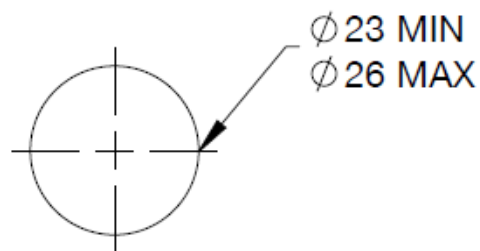
ROUGH-IN DIMENSIONS
